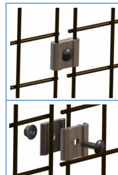
B. Screw Fence Connector
